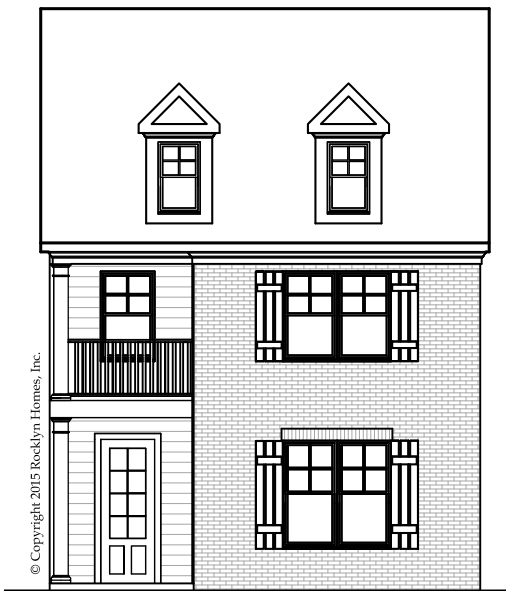
Elevation "AB"
