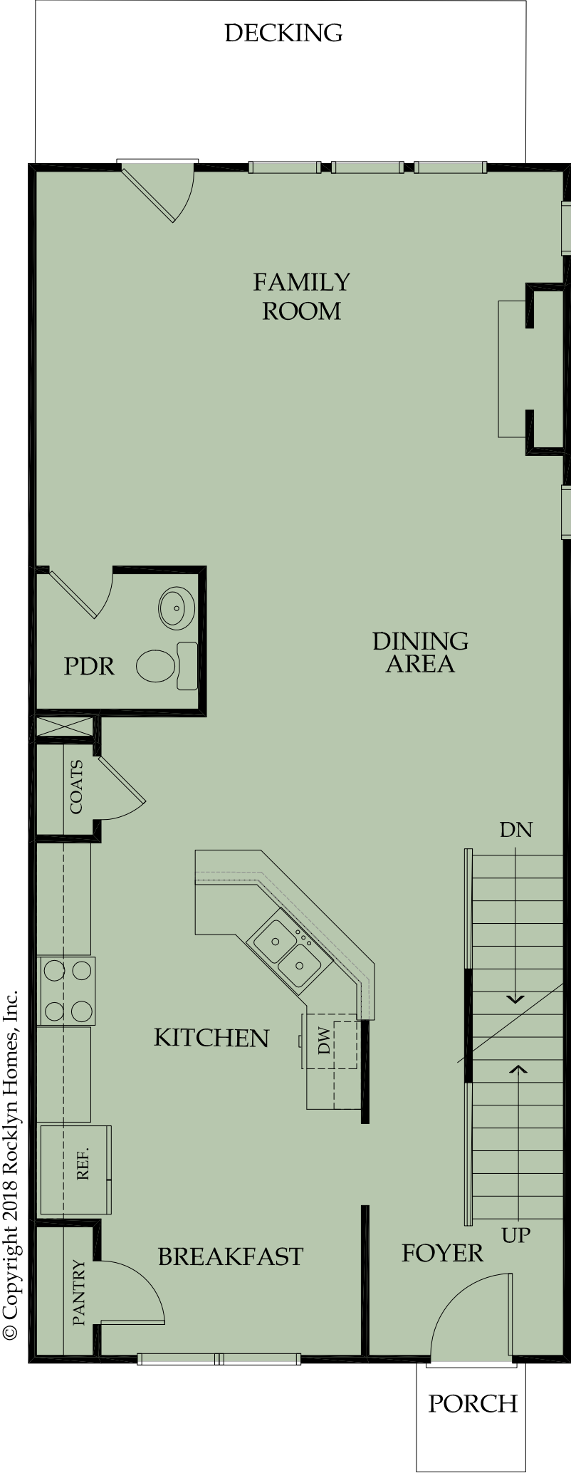
First Floor
