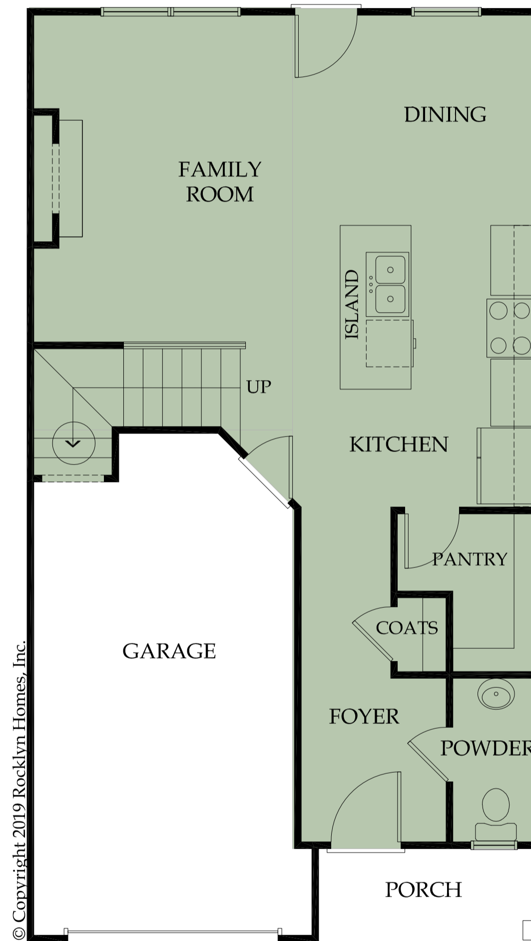
First Floor
