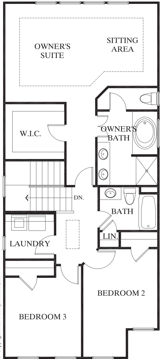
Second Floor
